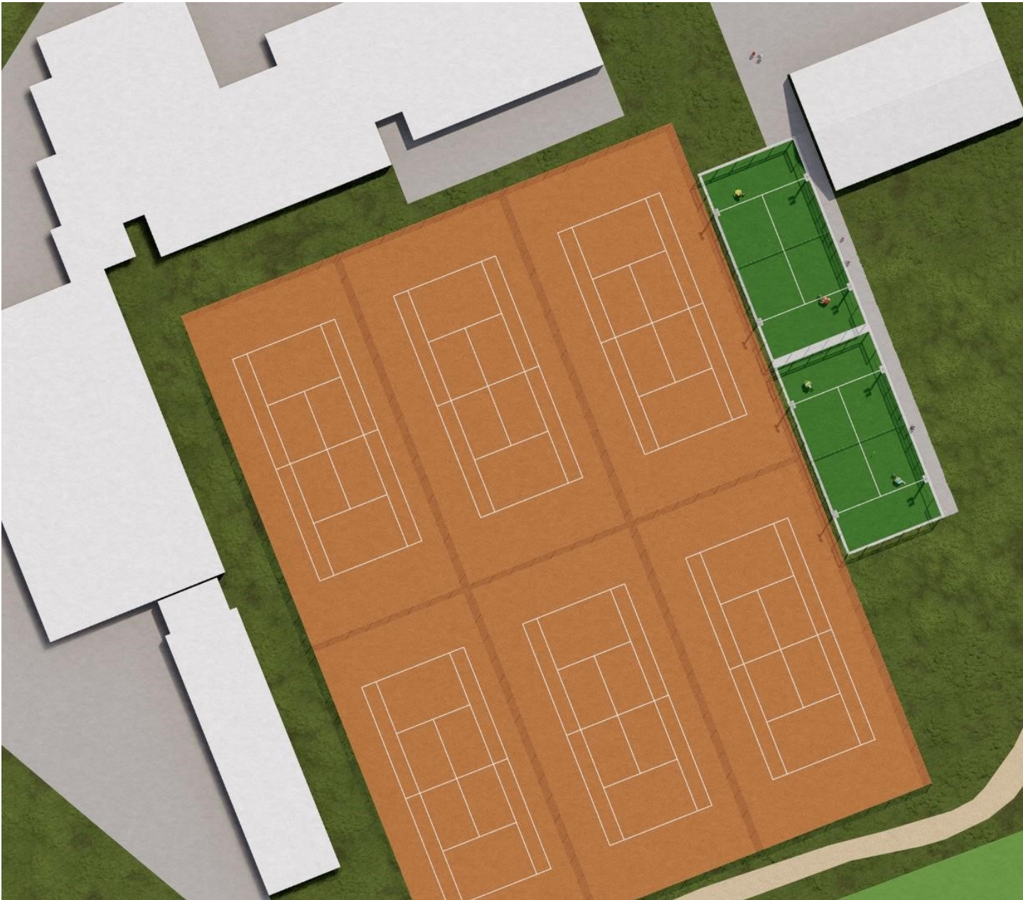
Bilag: Situationsplan for de to padelbaner
